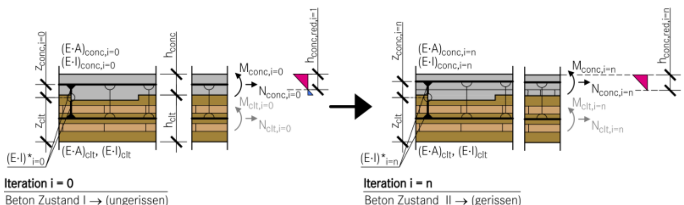
Abb. 6: Iteration
