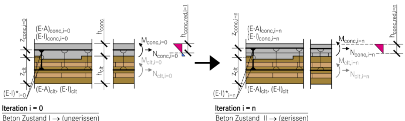
Abb. 6: Iteration
